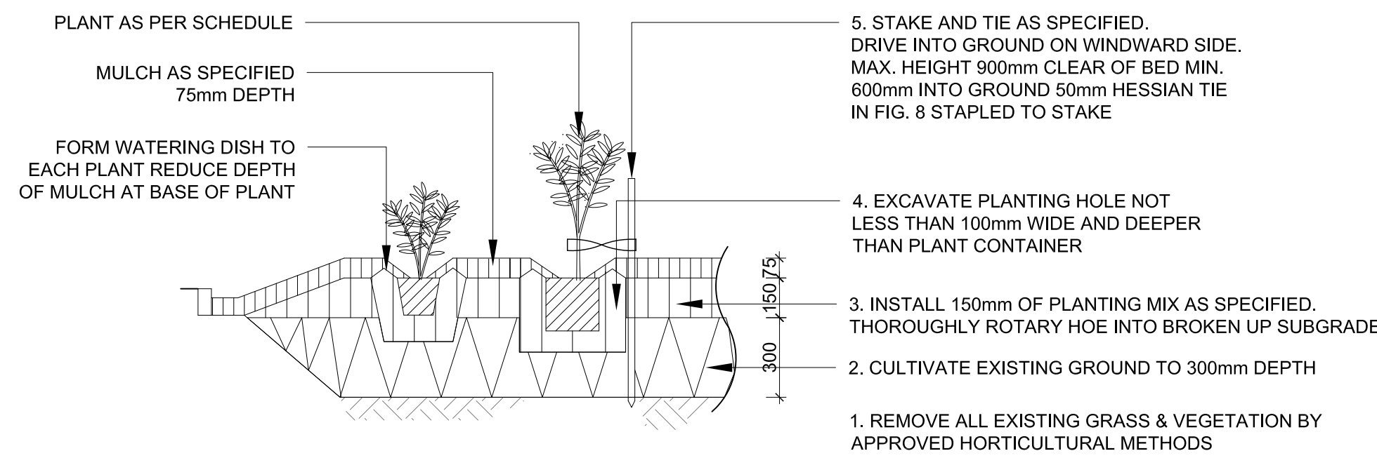
3 MASS PLANTING BED-NATURAL GROUND TYPICAL SECTION 1:20
