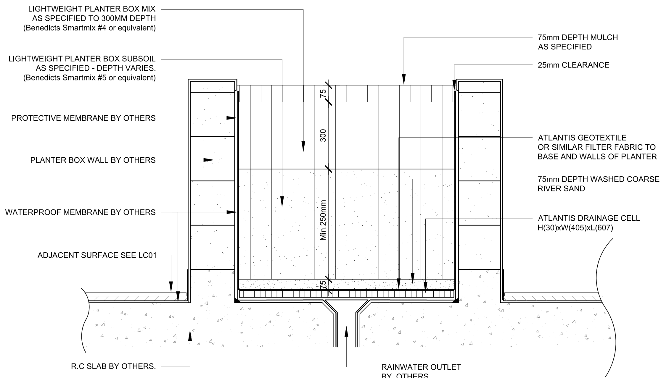
1 RAISED PLANTER BOX TYPICAL SECTION 1:10
