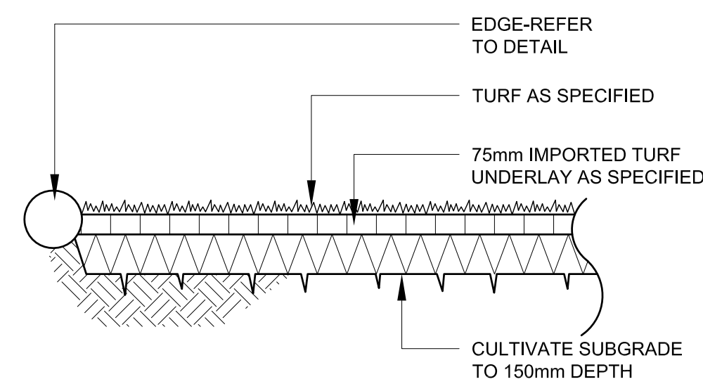
5 TURF ON GRADE SECTION 1:20
