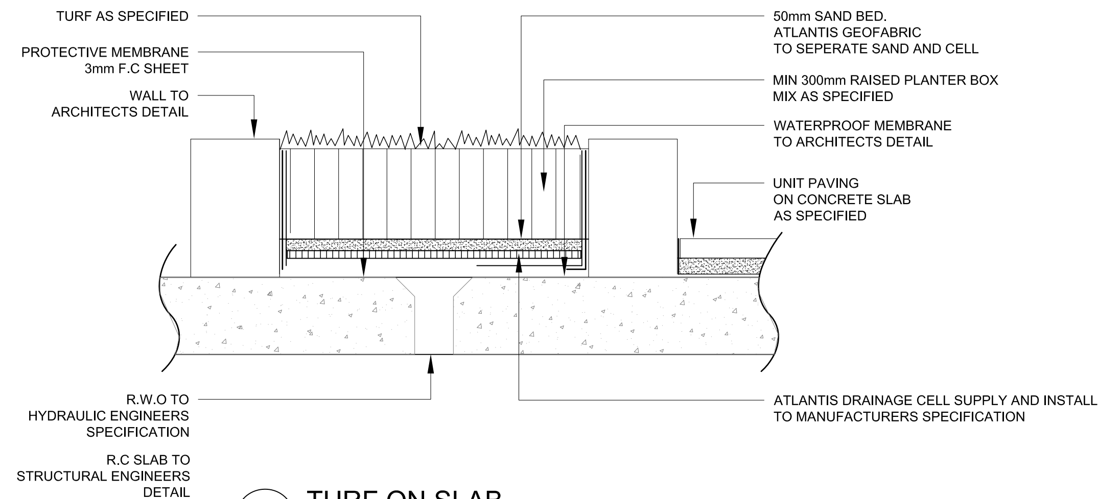
4 TURF ON SLAB TYPICAL SECTION 1:10
